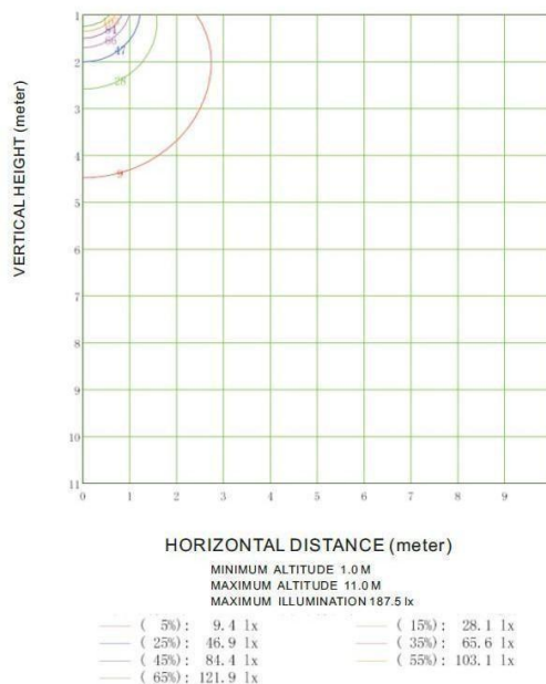
VERTICAL EQUILUMINOUS CURVE
